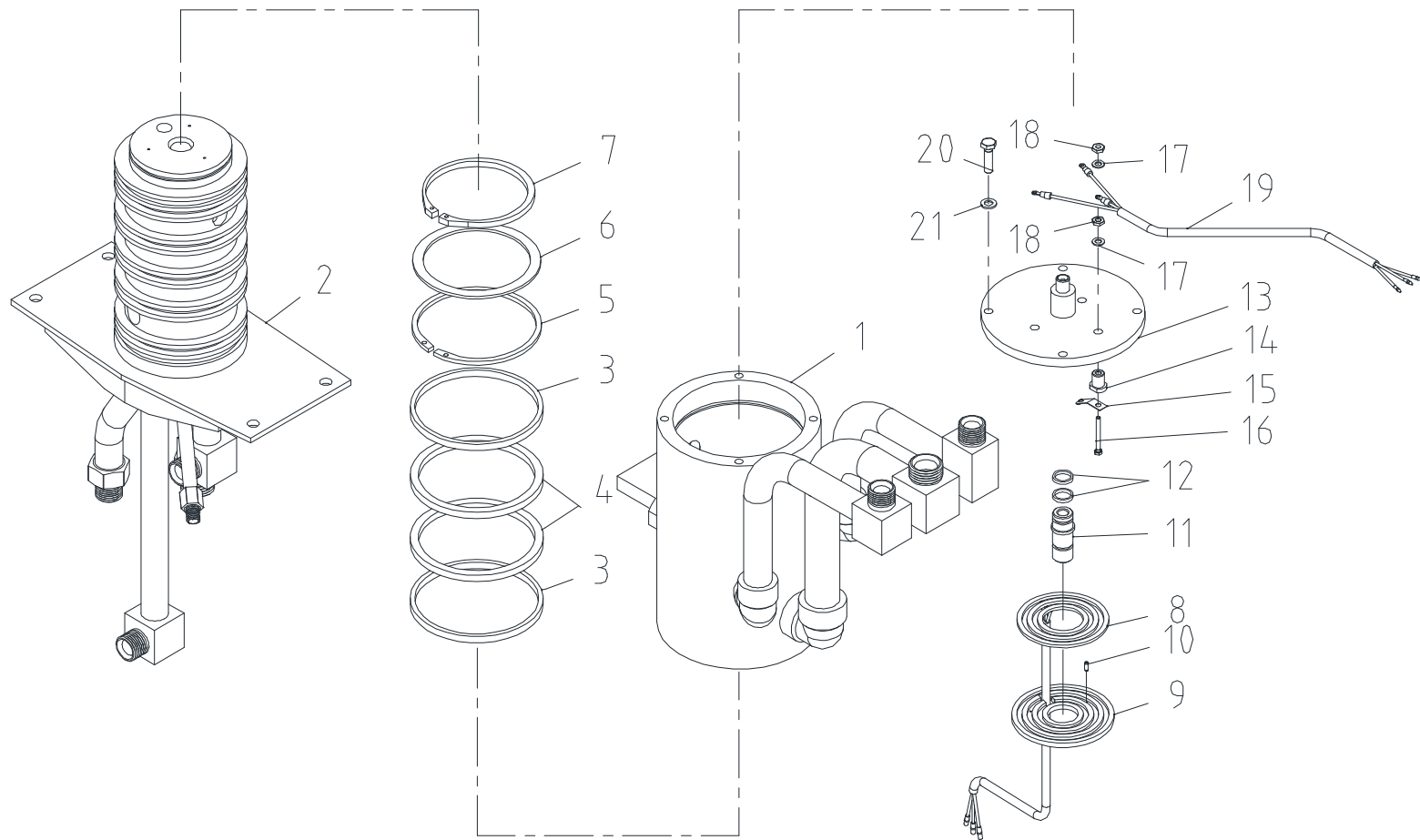
Fig. 3-1 SCS1216 ROTARY JOINT ASS'Y
