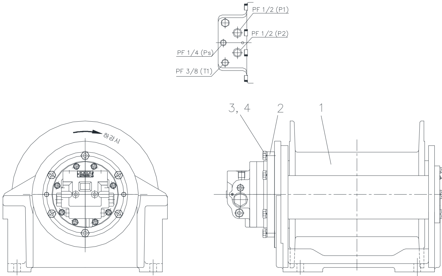
Fig. 2-1 SCS1216 2 SPEED WINCH ASS'Y
